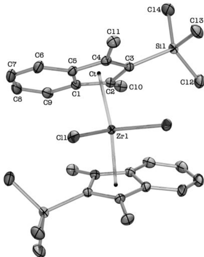
Figure 1. Refined crystallographic structure of bis[1,3-dimethyl-2-(trimethylsilyl)indenyl]zirconium dichloride ( 13b ). Hydrogen atoms are omitted for clarity. Thermal ellipsoids are at the 50% probability level.
