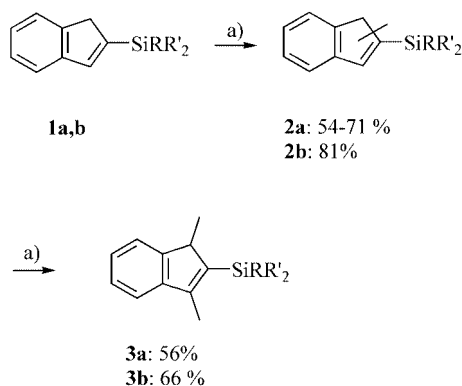
Scheme 1. General route towards 1,3-dialkyl-2-silylindenes. a) n BuLi, pentane, room temperature; MeI, diethyl ether, -40^{\circ}\text{C} . a: R = H, R' = Me. b: R = R' = Me. Yields are reported for the purified lithium salts of 3a and 3b , whereas spectroscopic data were obtained on the free ligands.
