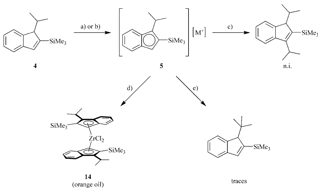
Scheme 2. Reactivity of 1-isopropyl-2-(trimethylsilyl)indene ( 4 ). a) n BuLi, pentane; b) potassium hydride, THF; c) 2-Iodopropane, diethyl ether/THF (n.i. = not isolated); d) \text{ZrCl}_4 , THF, -40^{\circ}\text{C} ; e) MeI, THF.
