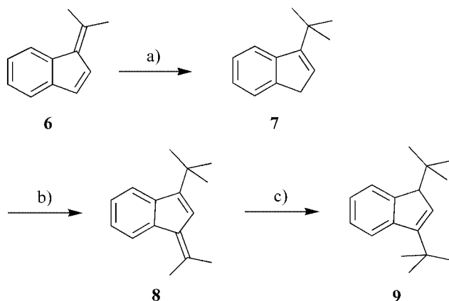
Scheme 3. A selective synthesis of 1,3-di- t Bu-indene ( 9 ). a) MeLi, Et 2 O, 0 °C or MeLi, pentane, 5 mol-% AlCl 3 / acidic work-up b) Pyrrolidine ex , acetone ex , MeOH, 48 h reflux; c) MeLi, Et 2 O, 6 h reflux.
