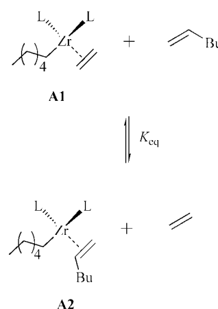
Scheme 5. Simplified representation of the active site with a polymer chain ( n -hexyl) attached: A1 with an ethene and A2 with a 1-hexene ligand. For clarity, the 1,3-dimethyl-2-TMS-indenyl ligands are abbreviated as “L” and charges are omitted.
